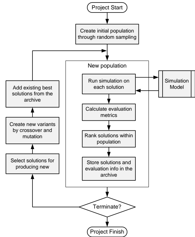
Figure 3: The EA process as implemented in JEA
